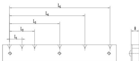
LS011
