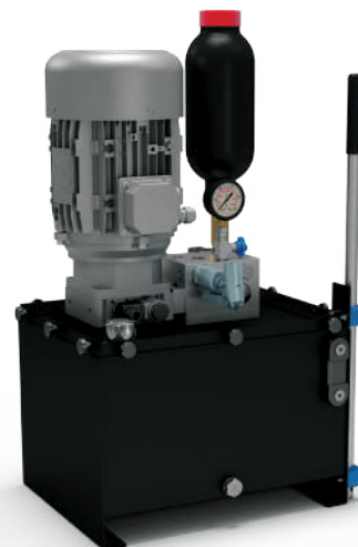
Serie 3 e 4 per Freni Negativi (N) e Positivi (P) Series 3 and 4 for Oil (P) and Spring Actuated Brakes (N)
