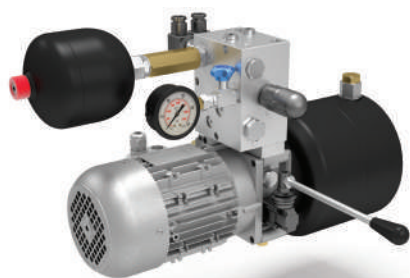
Serie 2 per Freni Negativi (N) e Positivi (P) Series 2 for Oil (P) and Spring Actuated Brakes (N)
